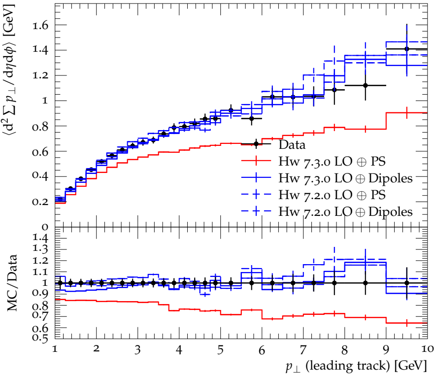
Away \Sigma p_{\perp} density vs. p_{\perp}^{\text{trk1}} , \sqrt{s} = 900 GeV, p_{\perp} > 100 MeV
