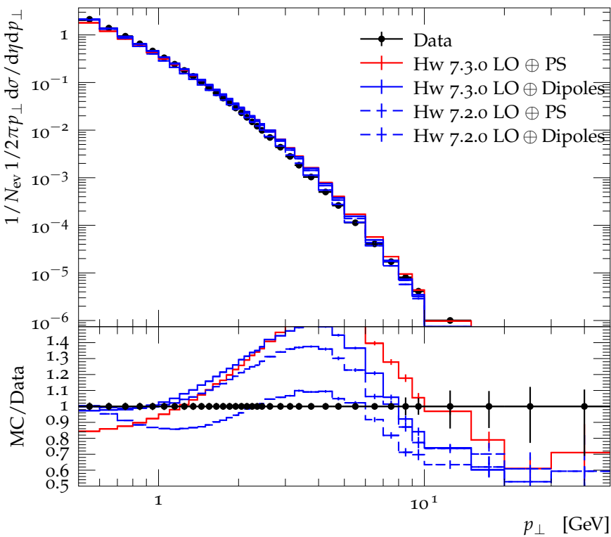
Charged particle p_{\perp} at 7 TeV, track p_{\perp} > 500 MeV, for N_{\text{ch}} \geq 6
