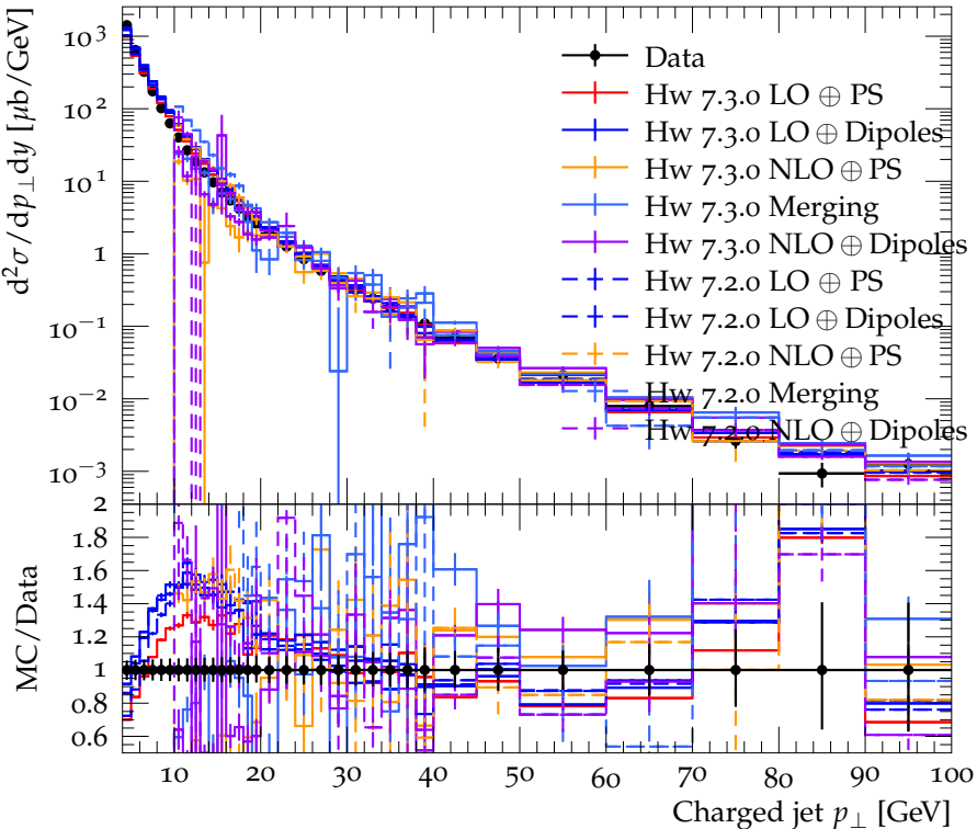
Charged jet cross section vs. p_{\perp} (anti- k_t , R = 0.4 , y 1.0-1.5)
