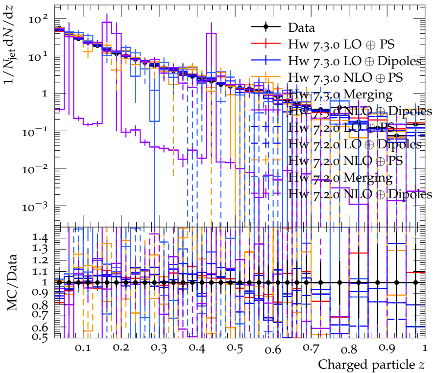
Charged jet z (anti- k_t , R = 0.4 , y 1.5-1.9, p_\perp 24.0-40.0)
