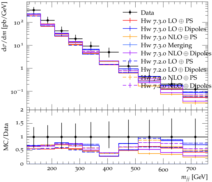
Dijet mass spectrum for |y| < 2.1 , anti- k_T , R = 0.4
