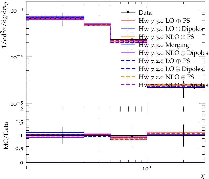
Dijet \chi for 110 < m_{jj} < 370 GeV, anti- k_T , R = 0.4
