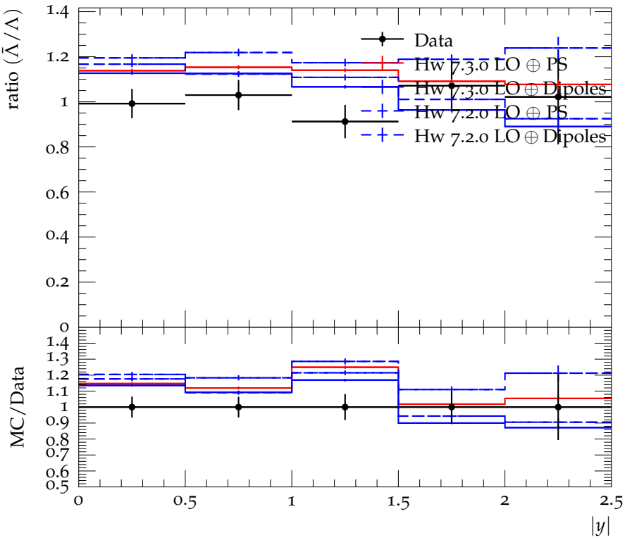
Production ratio of \bar{\Lambda} and \Lambda vs. |y| , \sqrt{s} = 900 GeV
