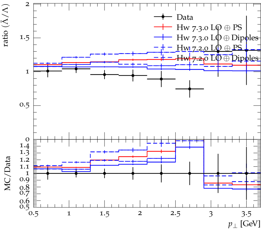
Production ratio of \bar{\Lambda} and \Lambda vs. p_{\perp} , \sqrt{s} = 900 GeV
