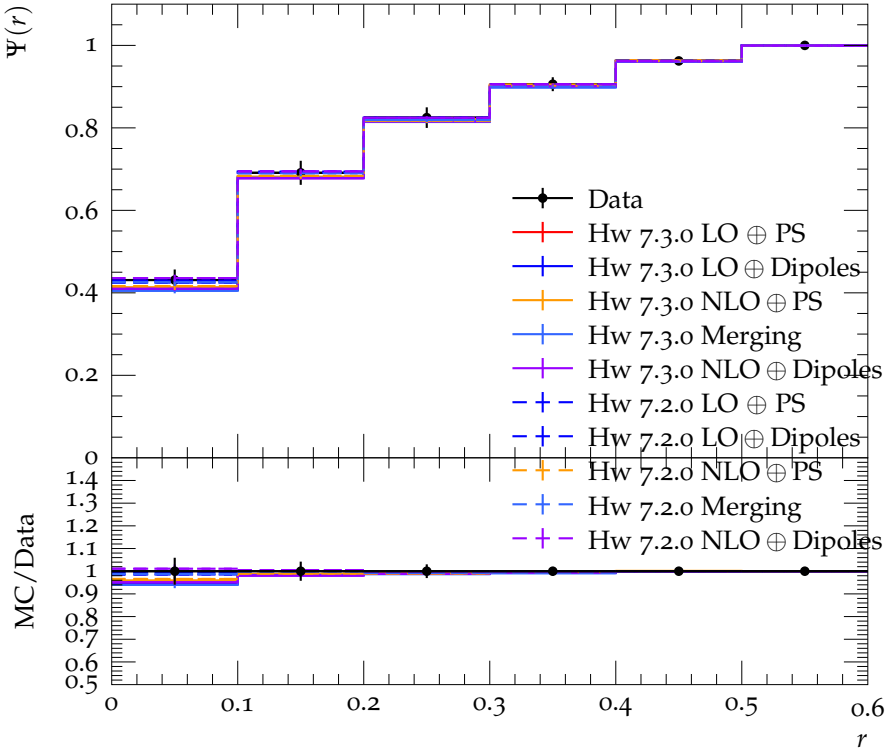
Jet shape \Psi for p_{\perp} \in 40\text{--}60\text{ GeV} , y \in 0.0\text{--}0.3
