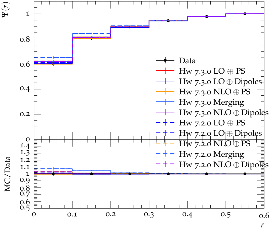
Jet shape \Psi for p_{\perp} \in 80\text{--}110\text{ GeV} , y \in 2.1\text{--}2.8
