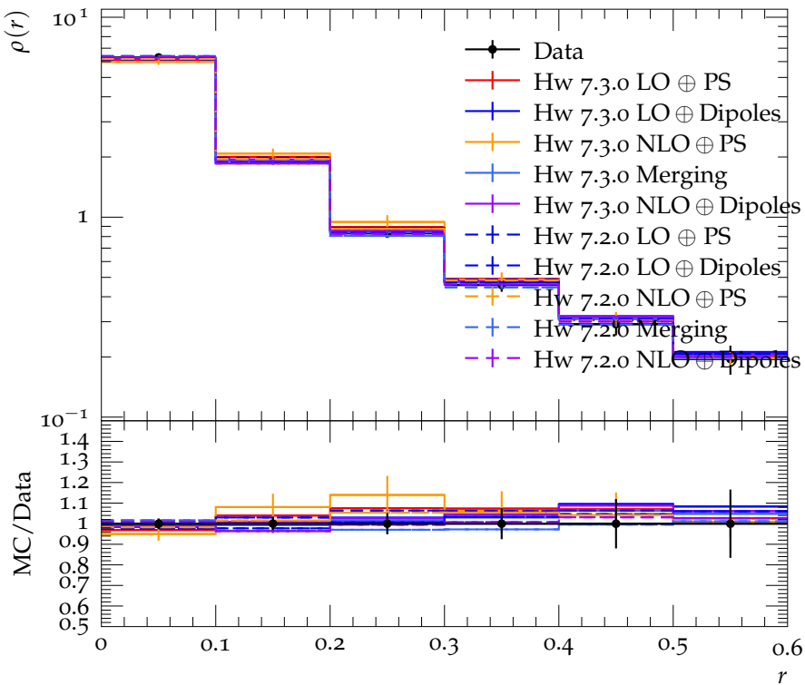
Jet shape \rho for p_{\perp} \in 110\text{--}160 GeV, y \in 0.0\text{--}2.8
