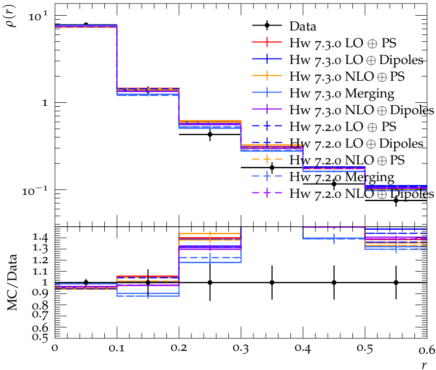
Jet shape \rho for p_{\perp} \in 400\text{--}500 GeV, y \in 0.3\text{--}0.8
