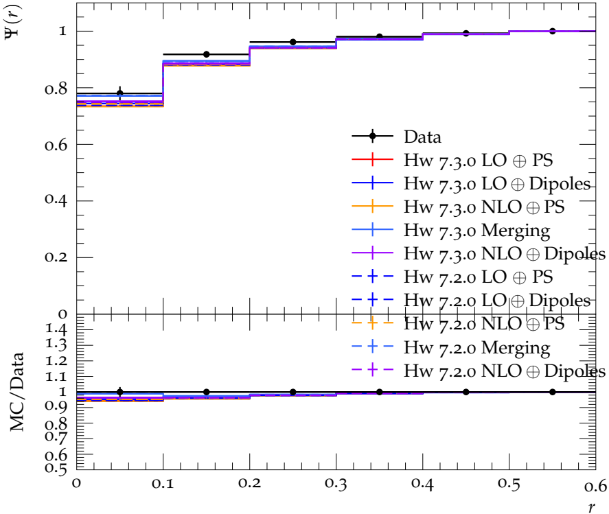
Jet shape \Psi for p_{\perp} \in 400\text{--}500 GeV, y \in 0.3\text{--}0.8
