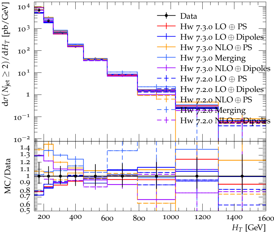
H_T for events with N_{\text{jet}} \geq 2 ( R = 0.4 )
