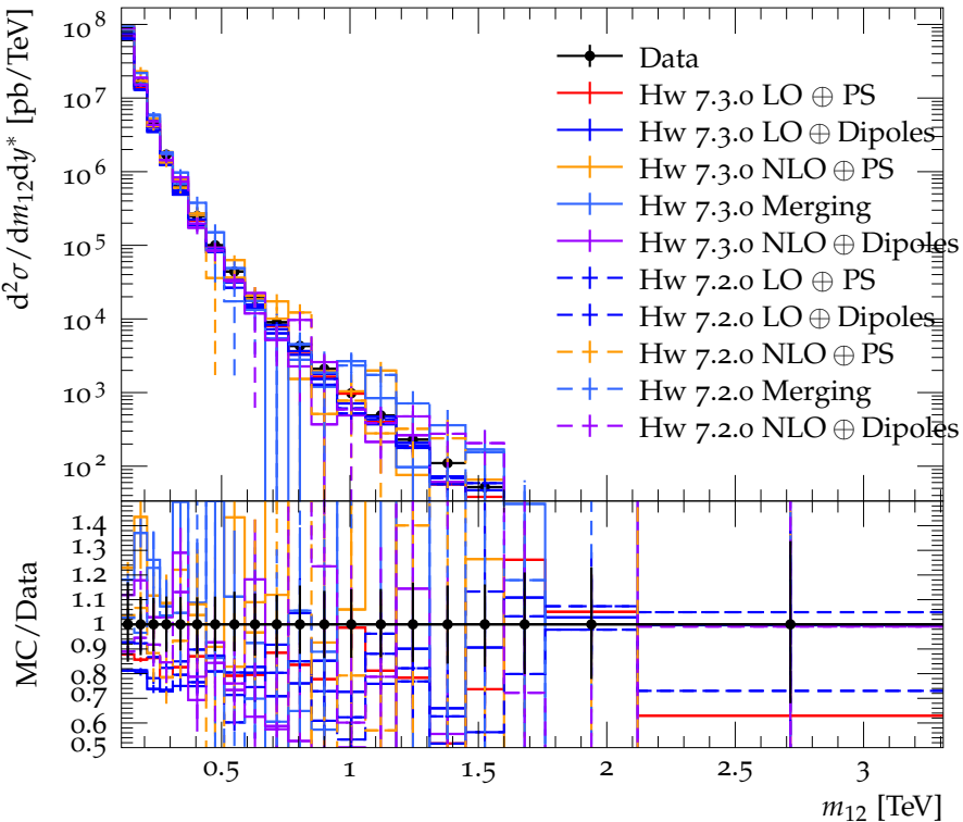
Dijet double-diff. x-section, anti- k_t 0.4 ( 0.5 \leq y^* < 1.0 )
