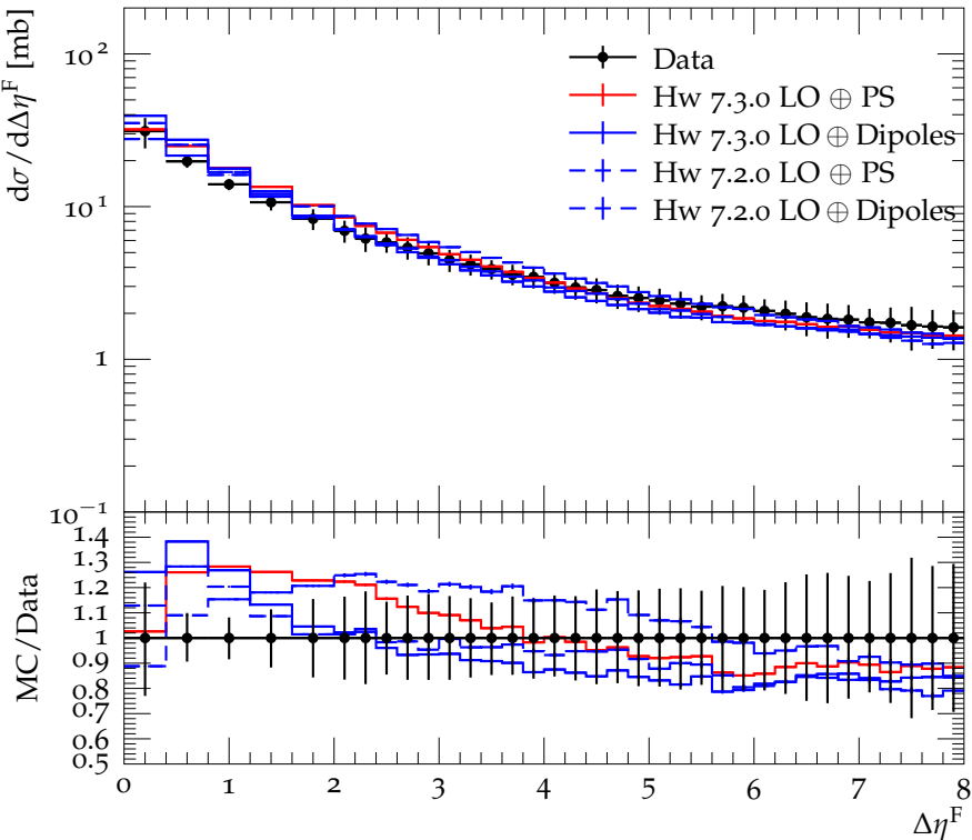
Rapidity gap size in \eta starting from \eta = \pm 4.9 , p_T > 800 MeV
