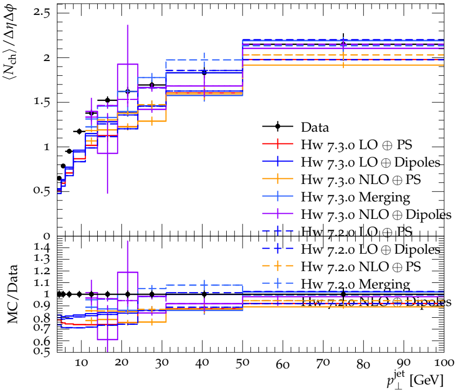
Mean N_{\text{ch}} vs. leading jet p_{\perp} , R = 0.8 , Away region
