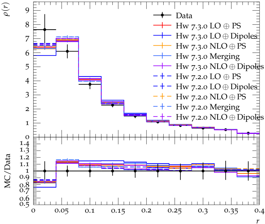
Differential jet shape for light-jets with 30 \text{ GeV} < p_T < 40 \text{ GeV}
