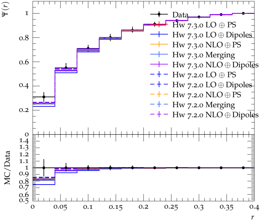
Integrated jet shape for light jets with 30 \text{ GeV} < p_T < 40 \text{ GeV}
