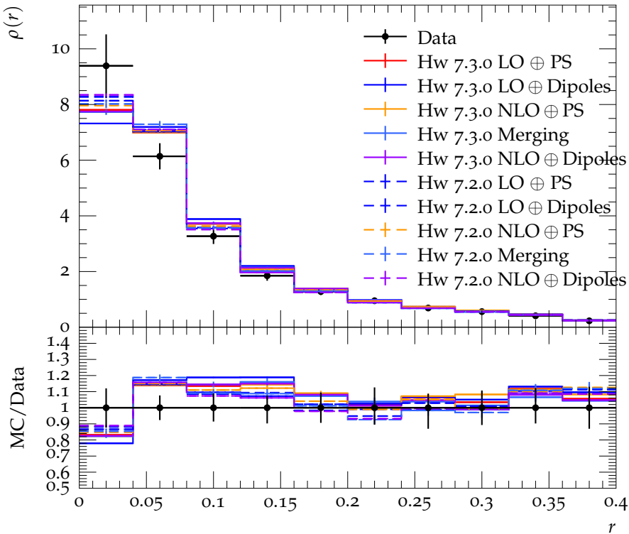
Differential jet shape for light-jets with 40 \text{ GeV} < p_T < 50 \text{ GeV}
