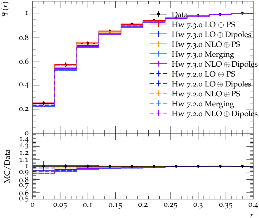
Integrated jet shape for b -jets with 50 \text{ GeV} < p_T < 70 \text{ GeV}
