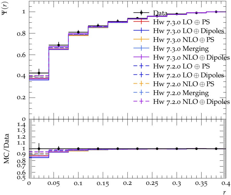
Integrated jet shape for light jets with 50 \text{ GeV} < p_T < 70 \text{ GeV}
