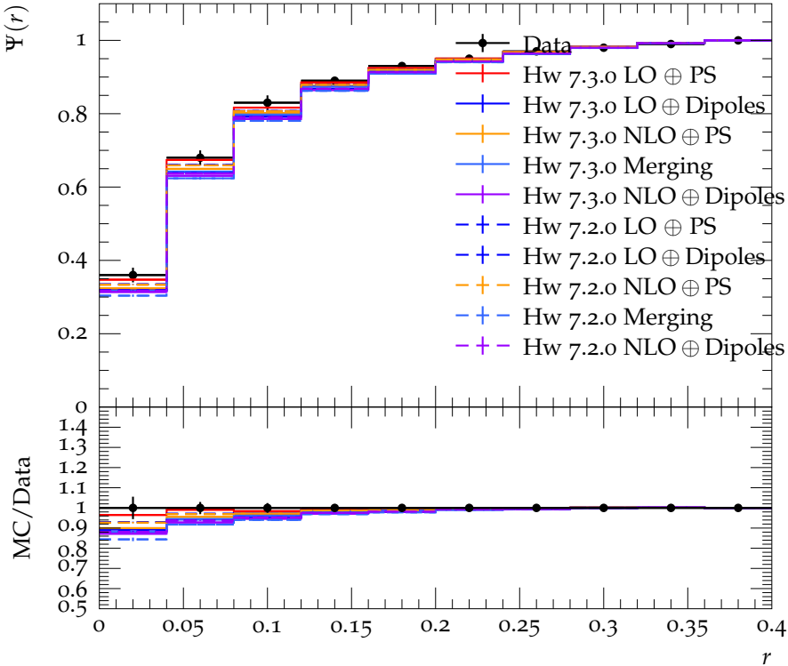
Integrated jet shape for b -jets with 70 \text{ GeV} < p_T < 100 \text{ GeV}
