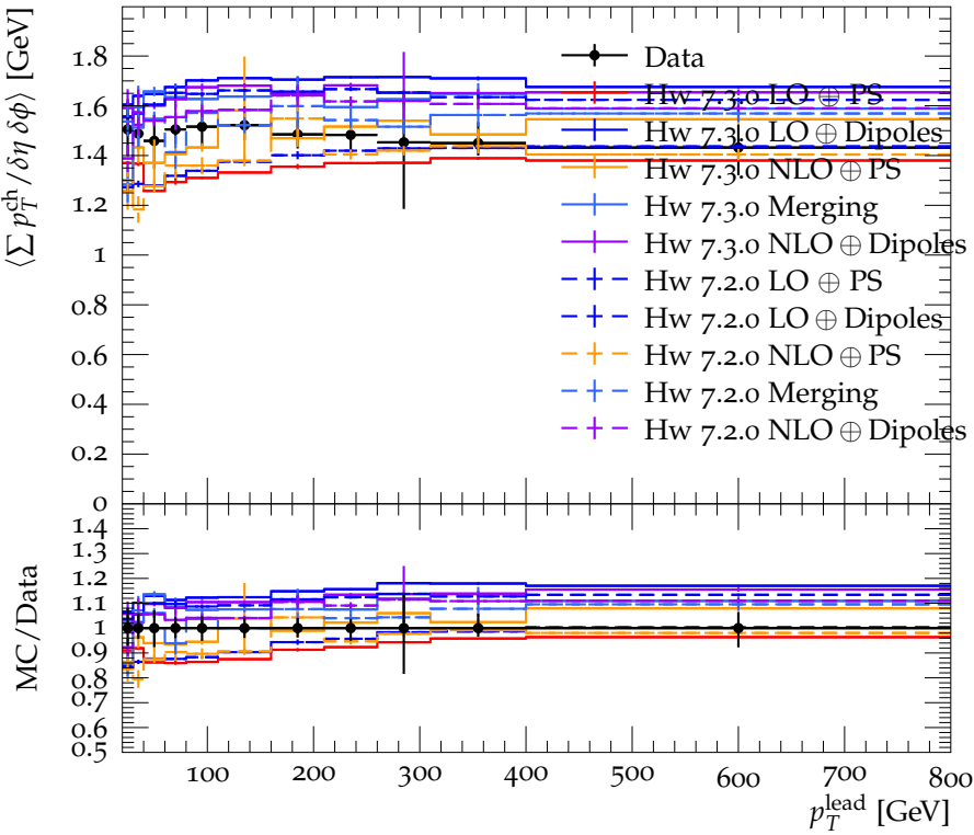
Trans-max \langle \sum p_T^{\text{ch}} / \delta\eta \delta\phi \rangle vs. p_T^{\text{lead}} in |\eta| < 2.5 in excl dijet events
