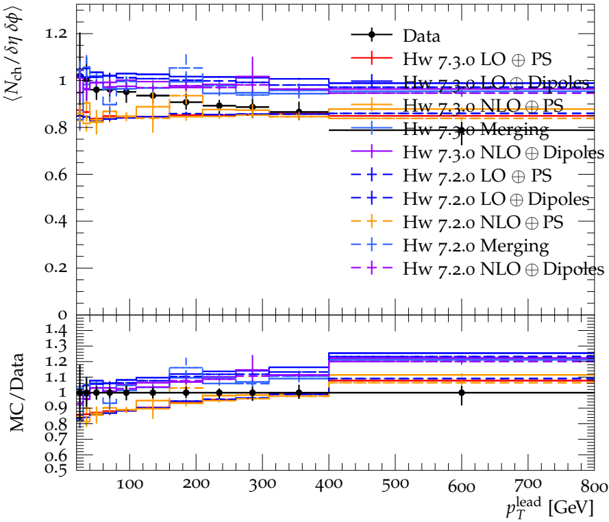
Transverse \langle N_{\text{ch}}/\delta\eta\delta\phi \rangle vs. p_T^{\text{lead}} in |\eta| < 2.5 in excl dijet events
