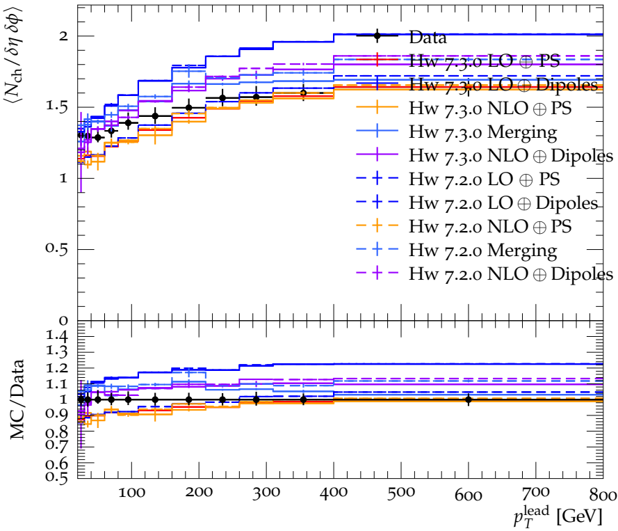
Trans-max \langle N_{\text{ch}}/\delta\eta\delta\phi \rangle vs. p_T^{\text{lead}} in |\eta| < 2.5 in incl jet events
