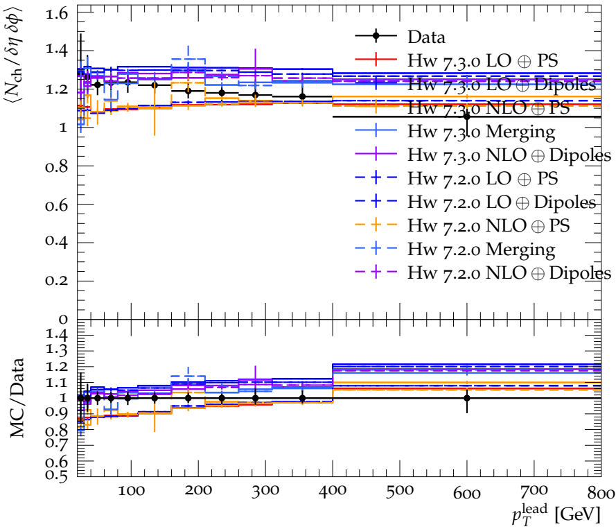
Trans-max \langle N_{\text{ch}}/\delta\eta\delta\phi \rangle vs. p_T^{\text{lead}} in |\eta| < 2.5 in excl dijet events
