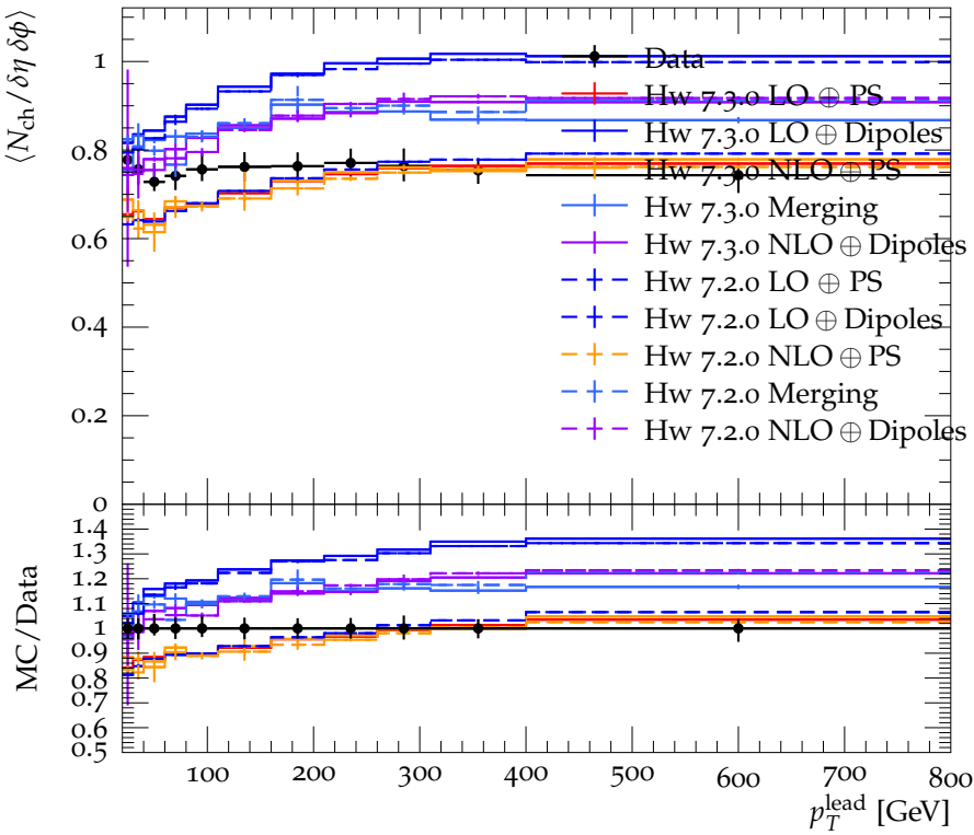
Trans-min \langle N_{\text{ch}}/\delta\eta\delta\phi \rangle vs. p_T^{\text{lead}} in |\eta| < 2.5 in incl jet events
