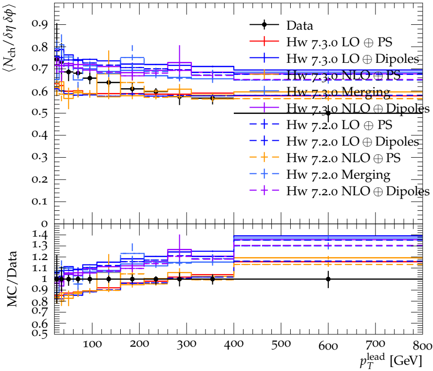
Trans-min \langle N_{\text{ch}}/\delta\eta\delta\phi \rangle vs. p_T^{\text{lead}} in |\eta| < 2.5 in excl dijet events
