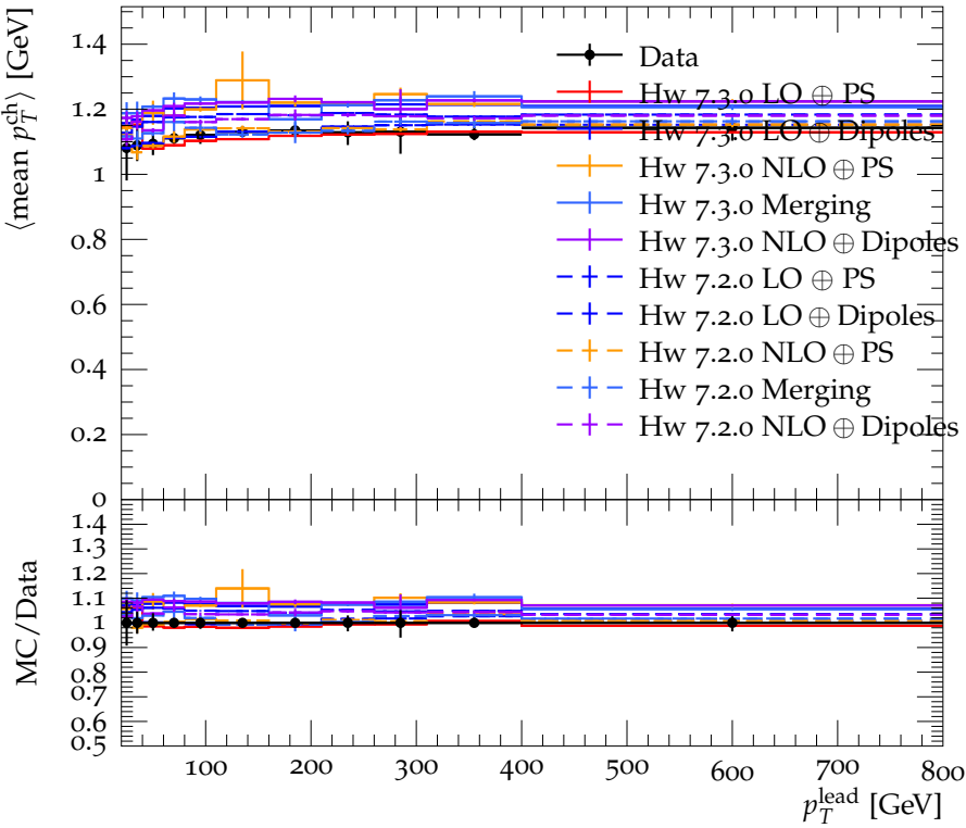
Transverse \langle \text{mean } p_T^{\text{ch}} \rangle vs. p_T^{\text{lead}} in |\eta| < 2.5 in excl dijet events
