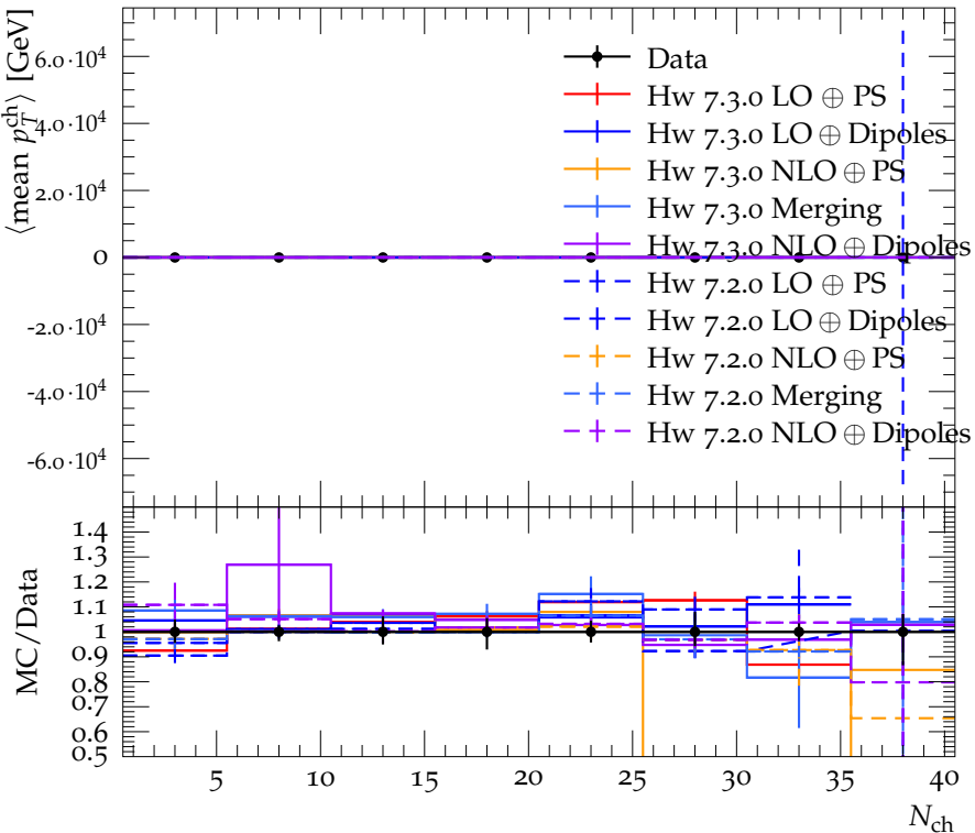
Transverse \langle \text{mean } p_T^{\text{ch}} \rangle vs. N_{\text{ch}} in |\eta| < 2.5 in excl dijet events
