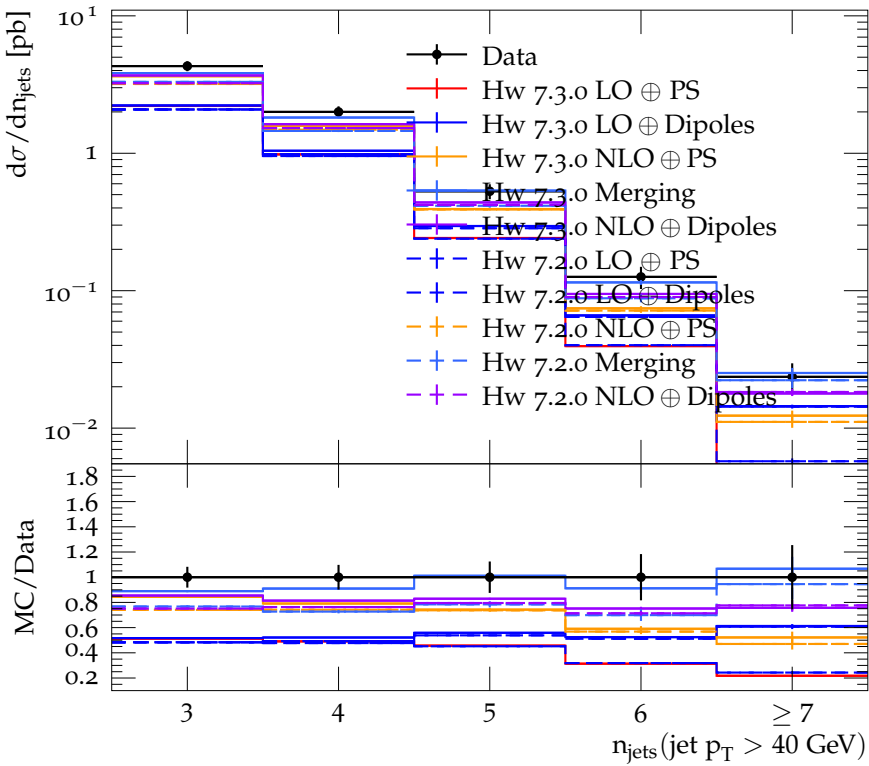
t\bar{t} cross-section vs. jet multiplicity for jets above 40 GeV
