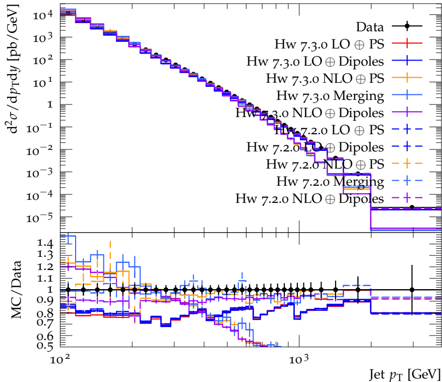
Inclusive jet cross section as a function of jet p_T ( 0.0 < |y| < 0.5 )
