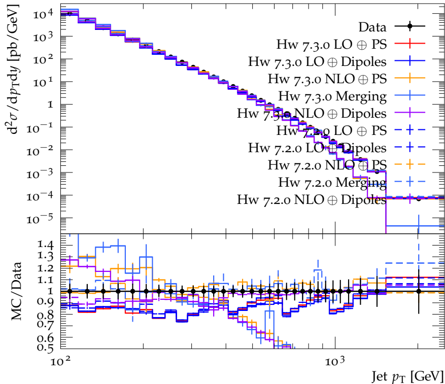
Inclusive jet cross section as a function of jet p_T ( 1.0 < |y| < 1.5 )
