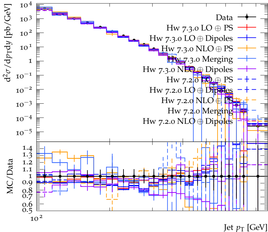
Inclusive jet cross section as a function of jet p_T ( 2.5 < |y| < 3.0 )
