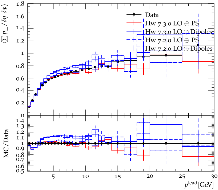
Mean \Sigma p_{\perp} density, trans-diff region
