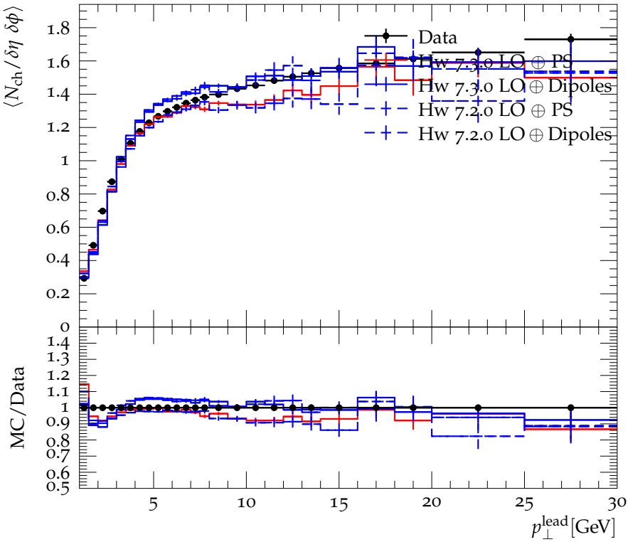
Mean charged-particle multiplicity density, towards region
