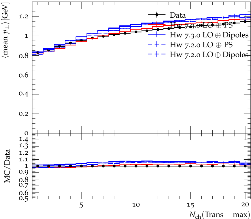
Mean average transverse momentum, trans-max region
