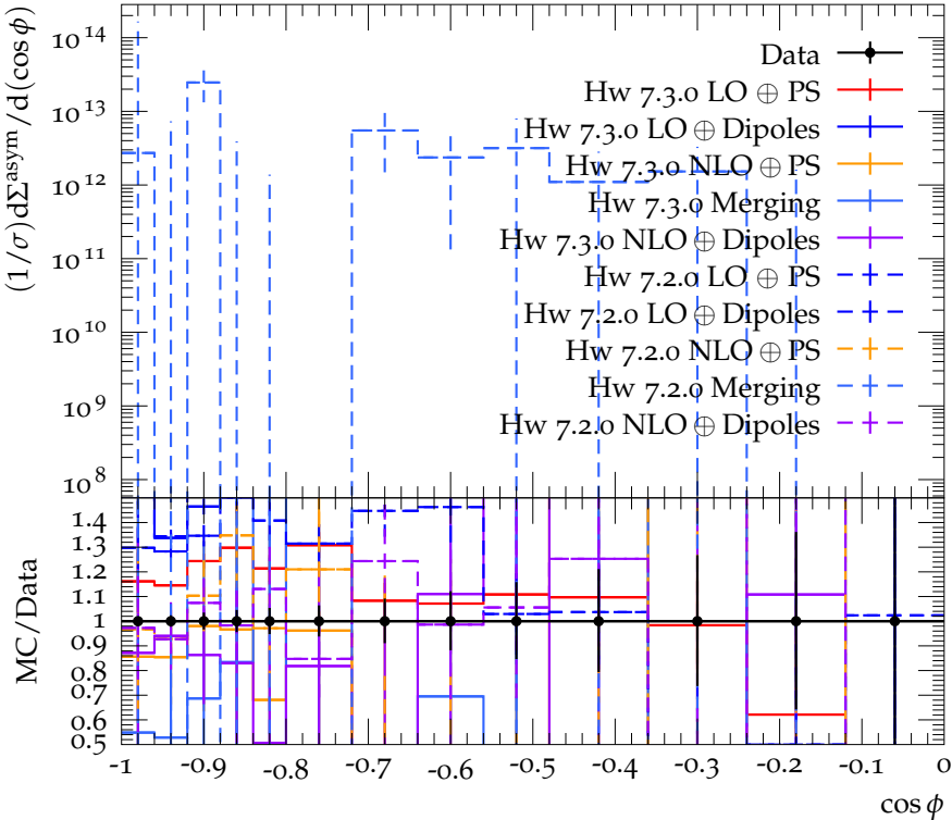
Transverse EEC asymmetry for 1000 \text{ GeV} < H_{T2} < 1100 \text{ GeV}
