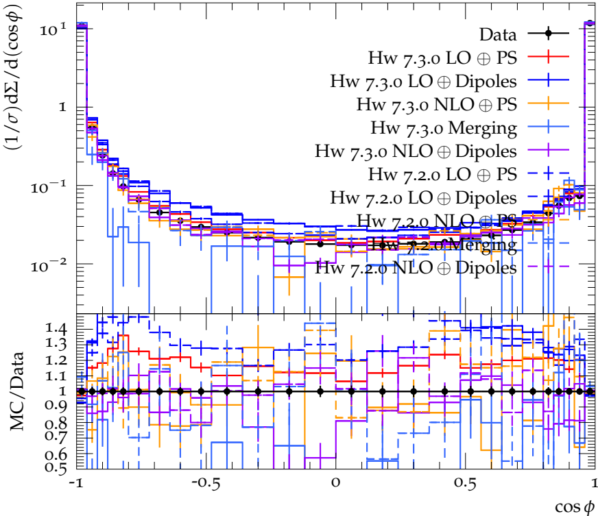
Transverse EEC for 1100 \text{ GeV} < H_{T2} < 1400 \text{ GeV}
