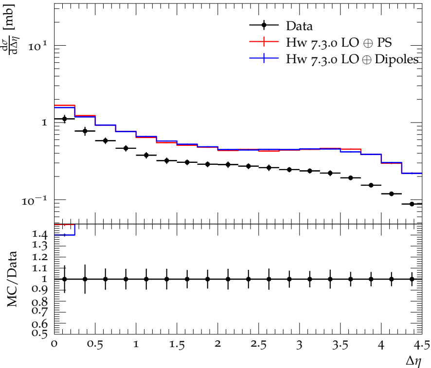
ALFA+ATLAS hadron-level differential SD cross section vs \Delta\eta
