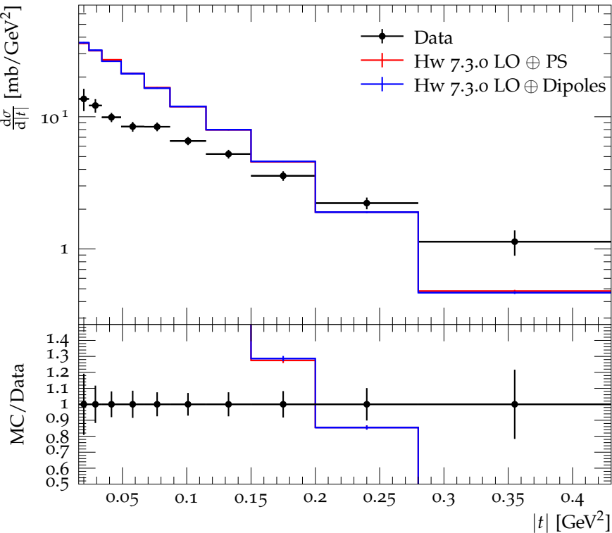
ALFA+ATLAS hadron-level differential SD cross section vs |t|
