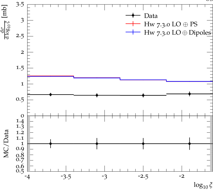
ALFA+ATLAS hadron-level differential SD cross section vs \log_{10} \xi
