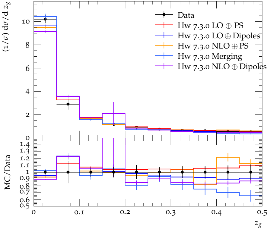
Dijet selection, Central jet, Cluster Based, Soft Drop \beta = 2.0, z_{cut} =
