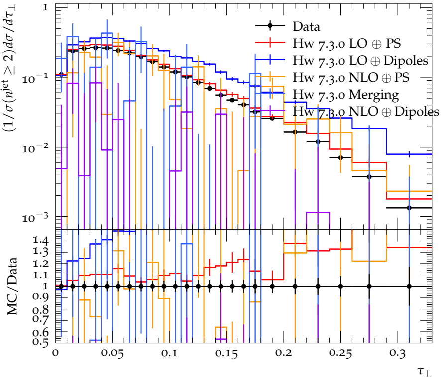
Transverse Thrust for n^{\text{jet}} = 5, H_{T2} > 2.0 TeV
