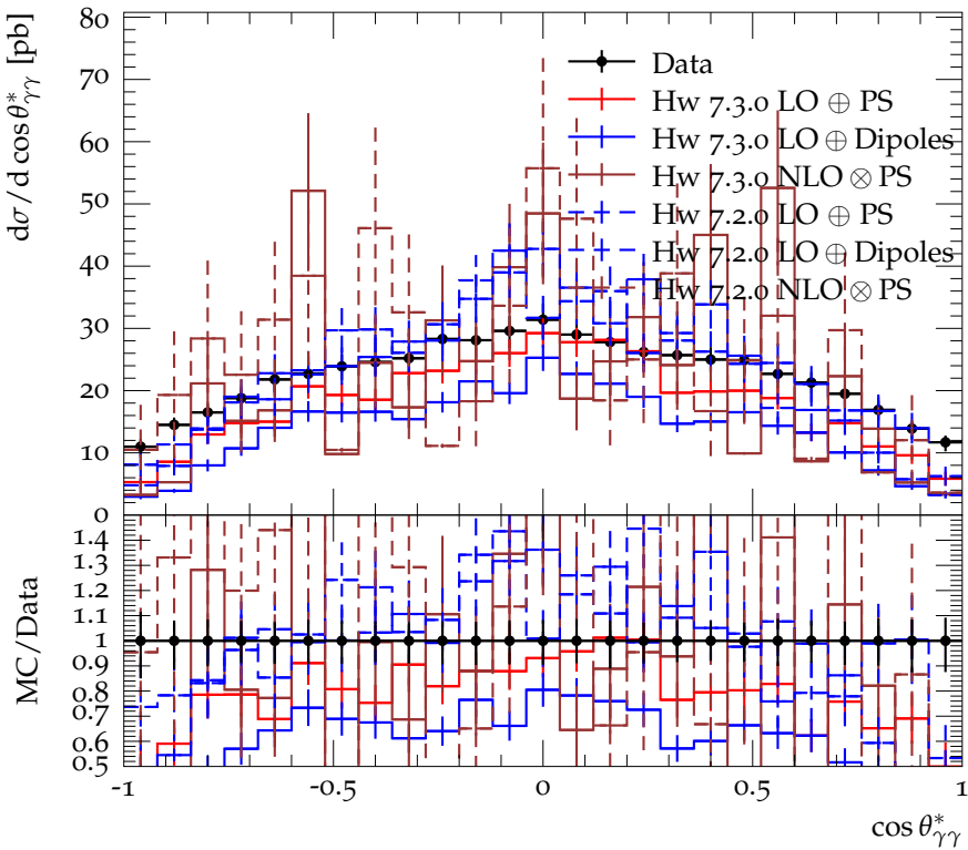
cross-section vs cosine of polar angle in Collins-Soper frame
