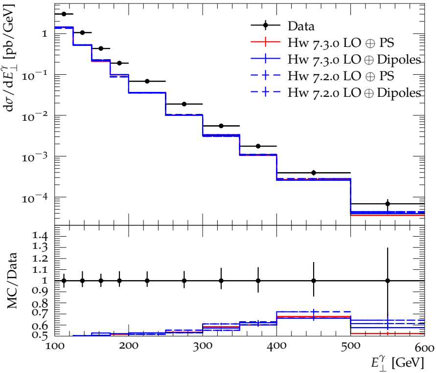
Transverse energy of isolated prompt photon, 1.52 \leq |\eta^\gamma| < 2.37
