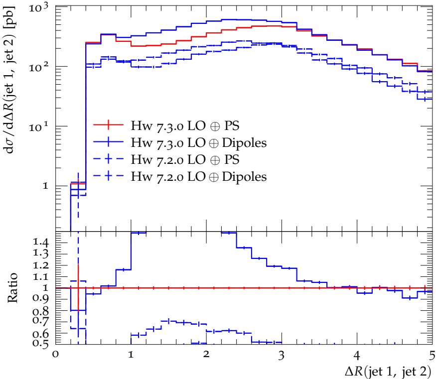
\Delta R separation between jets
