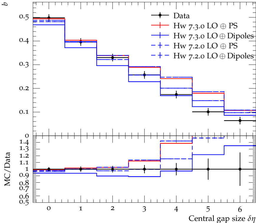
Forward-backward correlation b vs. gap size \sqrt{s} = 200 GeV
