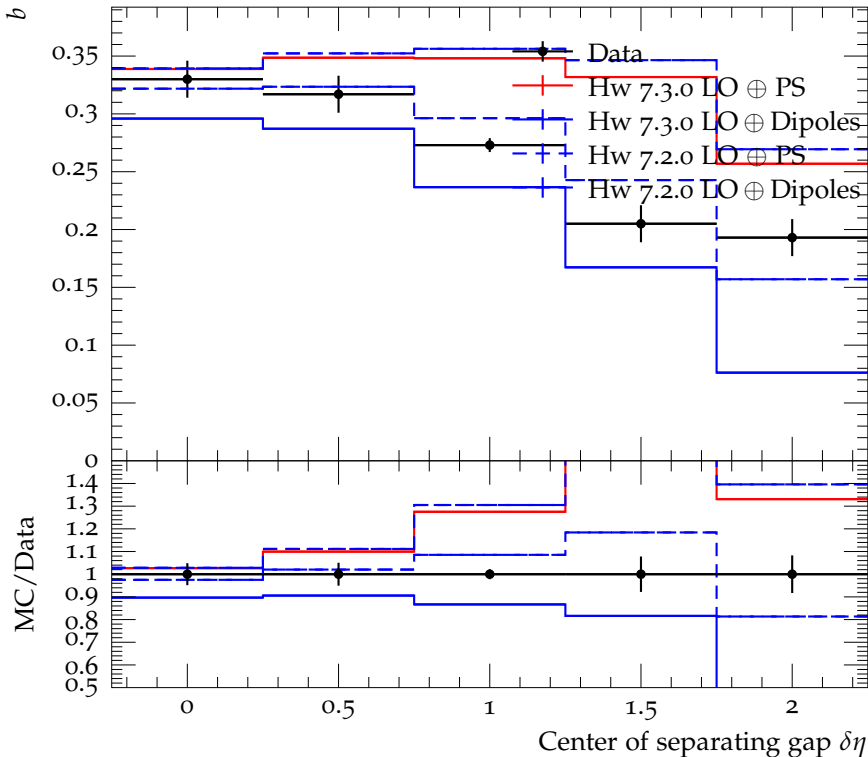
Forward-backward correlation b vs. gap center \sqrt{s} = 200 GeV
